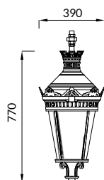
CHENONCEAUX II Suspended
